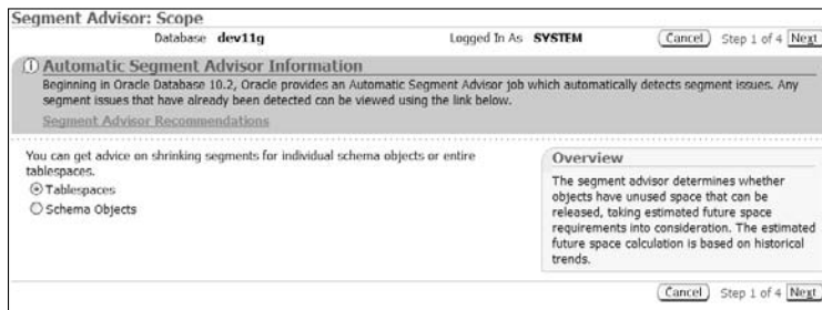
Figure 10-3: The Segment Advisor: Scope page lets you choose between analyzing segments or tablespaces.
