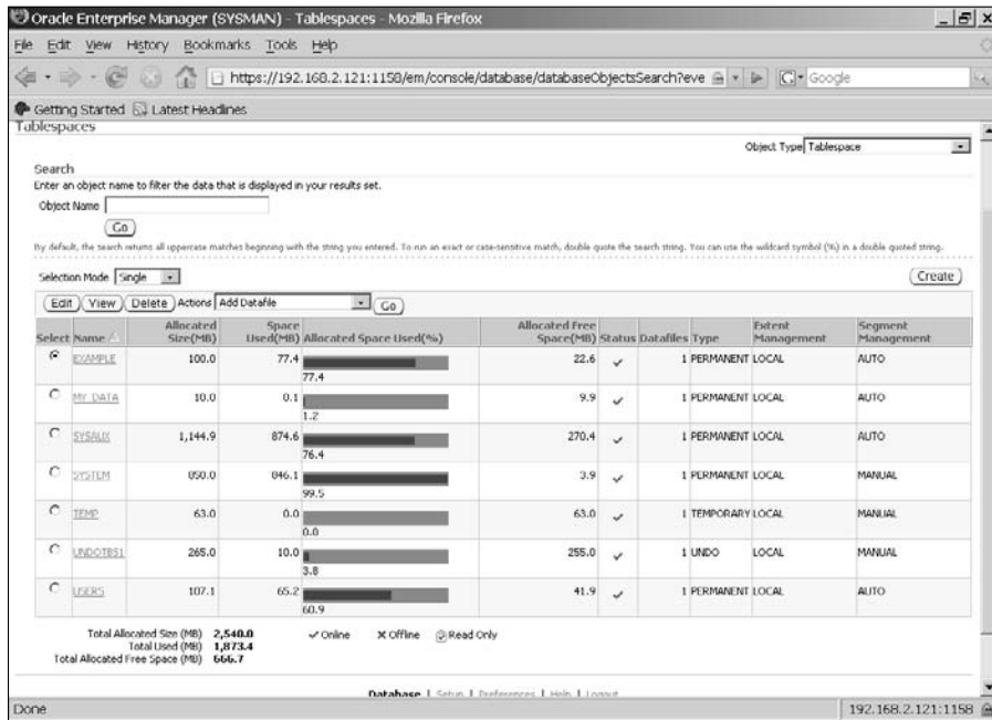
Figure 7-2: Tablespace management.
